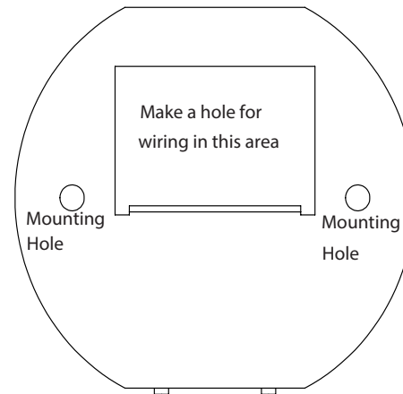
Round mounting diagram
